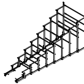
Sheridan Frame Assembly
